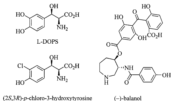
Figure 1. Representative examples of syn diastereoselectivity by DKR
