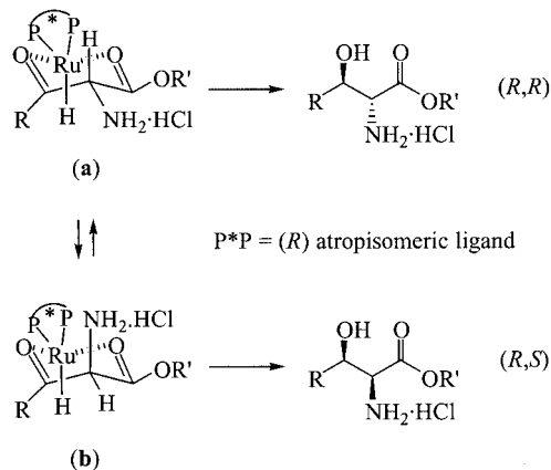
Scheme 6. Stereochemical model for anti stereoselectivity
