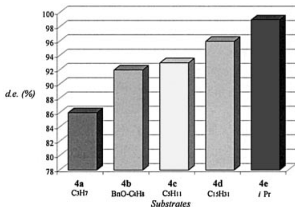
Scheme 5. Influence of the side chain on the diastereoselectivity of the hydrogenation reaction (reaction conducted with Ru-(S)-SYNPHOS® catalyst)
